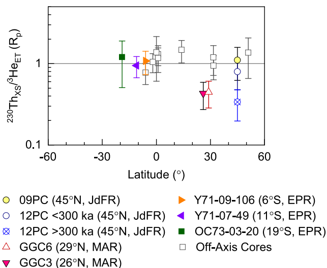
Fig. 6. Global compilation of core-averaged sedimentary ^{230}\text{Th}_{\text{XS}}/^{3}\text{He}_{\text{ET}} ratios with 1 standard deviation about each mean. Absolute ratios have been divided by the local production ratio ( R_p ) to allow for comparison between sites of different depths. Cores retrieved in proximity to the Juan de Fuca Ridge (JdFR), the Mid-Atlantic Ridge (MAR), and the East Pacific Rise (EPR; Lund et al., 2019) are highlighted with colored symbols. Off-axis data from Serno et al. (2015), McGee et al. (2010), and Marcantonio et al. (1995, 1996, 1999, 2001a, 2001b). Ratios are plotted on a log scale to highlight deviations from the production value of 1 R_p .
