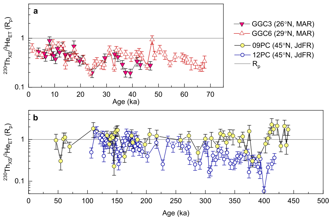
Fig. 4. Sedimentary ^{230}\text{Th}_{\text{XS}}/^{3}\text{He}_{\text{ET}} records for (a) the Mid-Atlantic Ridge (MAR; GGC3 and GGC6) and (b) the Juan de Fuca Ridge (JdFR; 09PC and 12PC). Absolute ratios have been divided by the local production ratio ( R_p ) to allow for comparison between sites of different depths. Mid-Atlantic Ridge ^{230}\text{Th}_{\text{XS}}/^{3}\text{He}_{\text{ET}} values are consistently lower than the expected production ratio ( 1 R_p ). On the Juan de Fuca Ridge, 12PC ^{230}\text{Th}_{\text{XS}}/^{3}\text{He}_{\text{ET}} values are increasingly lower than the production ratio with depth after \sim 300 ka. Note the change in axes scales between panels.
