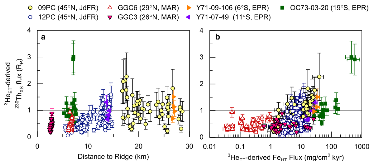
Fig. 7. Relationships between ^3\text{He}_{\text{ET}} -derived ^{230}\text{Th}_{\text{XS}} fluxes and (a) distance to the ridge-axis at time of deposition and (b) ^3\text{He}_{\text{ET}} -derived hydrothermal iron ( \text{Fe}_{\text{HT}} ) fluxes for sediments from the Mid-Atlantic Ridge (MAR; GGC3, GGC6), the Juan de Fuca Ridge (JdFR; 09PC, 12PC), and the East Pacific Rise (EPR; OC73-3-20, Y71-09-106, Y71-07-49; Lund et al., 2019). \text{Fe}_{\text{HT}} fluxes are calculated using ^3\text{He}_{\text{ET}} -derived mass accumulation rates. Absolute ^3\text{He}_{\text{ET}} -derived ^{230}\text{Th}_{\text{XS}} fluxes have been divided by the local ^{230}\text{Th}_{\text{XS}} production rate ( R_{\text{P}} ) to allow for comparison between sites of different depths. For consistency of comparison, ^3\text{He}_{\text{ET}} -derived fluxes in East Pacific Rise records have been recalculated using a ^3\text{He}_{\text{ET}} influx of 8.0 \pm 1.2 \times 10^{-13} cc STP \text{cm}^{-2} \text{kyr}^{-1} . GGC6 samples with negative \text{Fe}_{\text{HT}} flux values are excluded from b.
