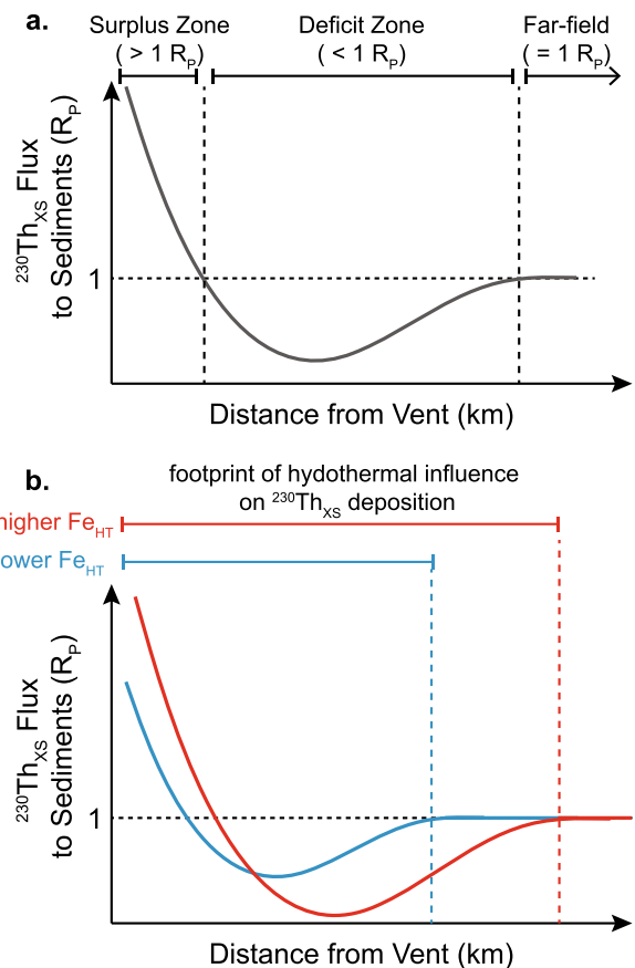
Fig. 10. Conceptual diagram illustrating the variable effects of hydrothermal scavenging of seawater ^{230}\text{Th}_{\text{XS}} on ^{230}\text{Th}_{\text{XS}} deposition rates in near-ridge sediments. (a) Closest to the vent, ^{230}\text{Th}_{\text{XS}} deposition rates to surplus zone sediments are higher than the overlying water column production rate ( R_p ); farther from the vent site, ^{230}\text{Th}_{\text{XS}} deposition rates to deficit zone sediments are lower than the overlying water column production rate; beyond the footprint of hydrothermal influence, ^{230}\text{Th}_{\text{XS}} deposition rates in far-field sediments match the water column production rate. (b) Higher levels of hydrothermal Fe ( \text{Fe}_{\text{HT}} ) output at the vent site drive enhanced hydrothermal scavenging and result in a larger hydrothermal footprint in sedimentary ^{230}\text{Th}_{\text{XS}} .
