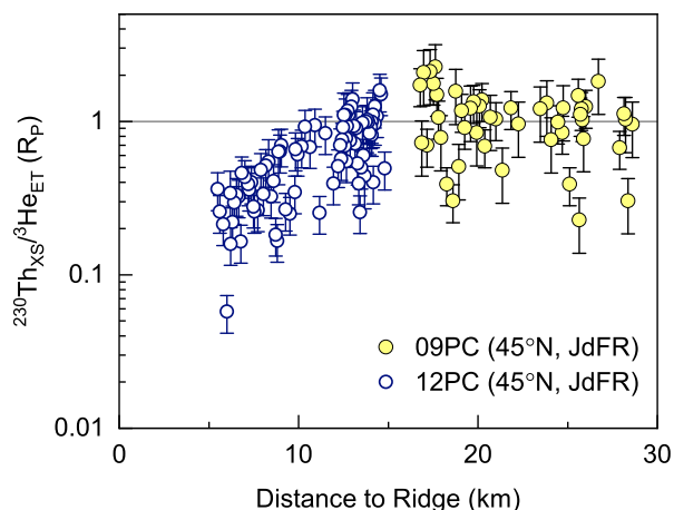
Fig. 5. Juan de Fuca Ridge (JdFR; 09PC, 12PC) ^{230}\text{Th}_{\text{XS}}/^{3}\text{He}_{\text{ET}} values as a function of distance to the spreading axis of the nearby mid-ocean ridge. Absolute ratios have been divided by the local production ratio ( R_p ) to allow for comparison between sites of different depths. Paleo-distance is estimated assuming a Cleft Segment half-spreading rate of 30 mm/yr (Govers and Meijer, 2001). Juan de Fuca Ridge ^{230}\text{Th}_{\text{XS}}/^{3}\text{He}_{\text{ET}} values decrease with increasing proximity to the ridge. Ratios are plotted on a log scale to highlight deviations from the production value of 1 R_p .
