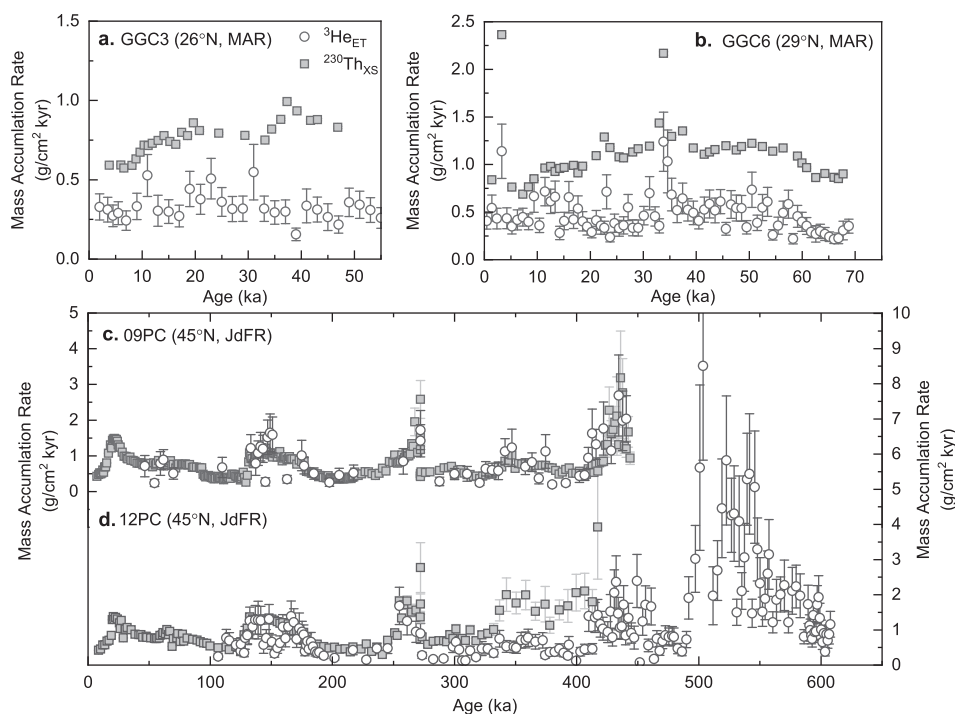
Fig. 3. Mass accumulation rate records derived using {}^3\text{He}_{\text{ET}} (open circles) and {}^{230}\text{Th}_{\text{XS}} (gray squares) for sediments from (a,b) the Mid-Atlantic Ridge (MAR; GGC3 and GGC6) and (c,d) the Juan de Fuca Ridge (JdFR; 09PC and 12PC).
