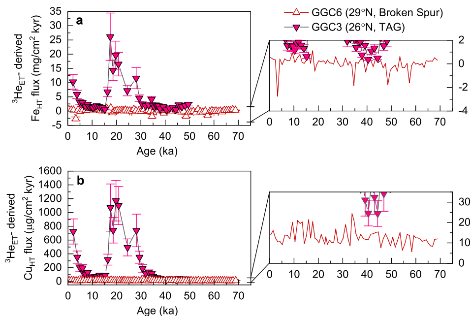
Fig. 2. Comparison of hydrothermal fluxes in Mid-Atlantic Ridge sediments. (a) Hydrothermal iron ( \text{Fe}_{\text{HT}} ) and (b) hydrothermal copper ( \text{Cu}_{\text{HT}} ) fluxes for GGC6 (Broken Spur Segment, 29°N; open triangles) and GGC3 (TAG Segment, 26°N, closed triangles; Middleton et al. 2016). Insets highlight GGC6 flux records on a zoomed-in y-axis. GGC6 symbols and error bars excluded from insets for clarity. Low GGC6 \text{Fe}_{\text{HT}} and \text{Cu}_{\text{HT}} fluxes suggest weak hydrothermal deposition. Negative values reflect uncertainty in the lithogenic correction applied.
