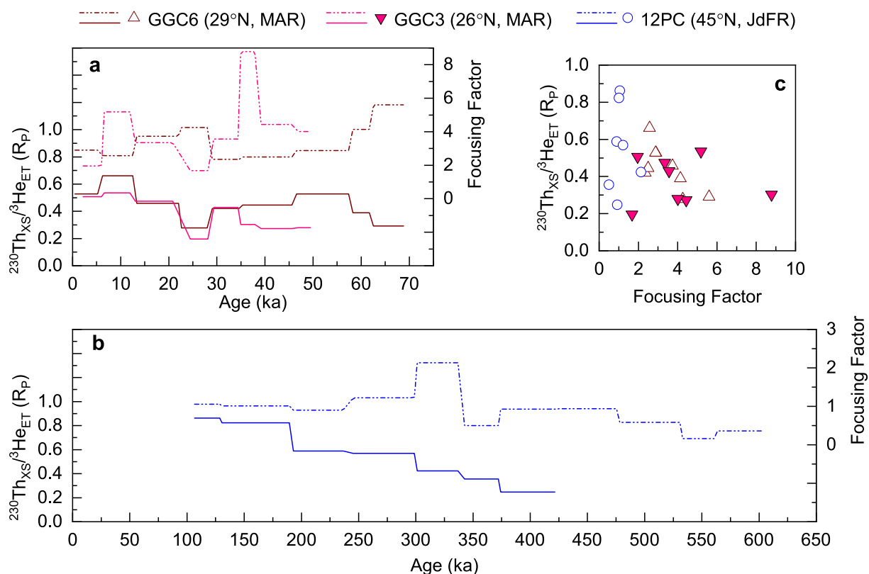
Fig. 8. ^3\text{He}_{\text{ET}} -derived sediment focusing factors (dashed lines) and average ^{230}\text{Th}_{\text{XS}}/^3\text{He}_{\text{ET}} values between age model tie points (solid lines) for near-axis sediments from (a) the Mid-Atlantic Ridge (MAR; GGC3, GGC6) and (b) the Juan de Fuca Ridge (JdFR; 12PC). Absolute ^{230}\text{Th}_{\text{XS}}/^3\text{He}_{\text{ET}} ratios have been divided by the local production ratio ( R_p ). (c) Direct comparison of ^{230}\text{Th}_{\text{XS}}/^3\text{He}_{\text{ET}} and focusing factor for GGC3 (closed triangles), GGC6 (open triangles), and 12PC (open circles). There are no clear relationships between sediment focusing and ^{230}\text{Th}_{\text{XS}}/^3\text{He}_{\text{ET}} variability.
