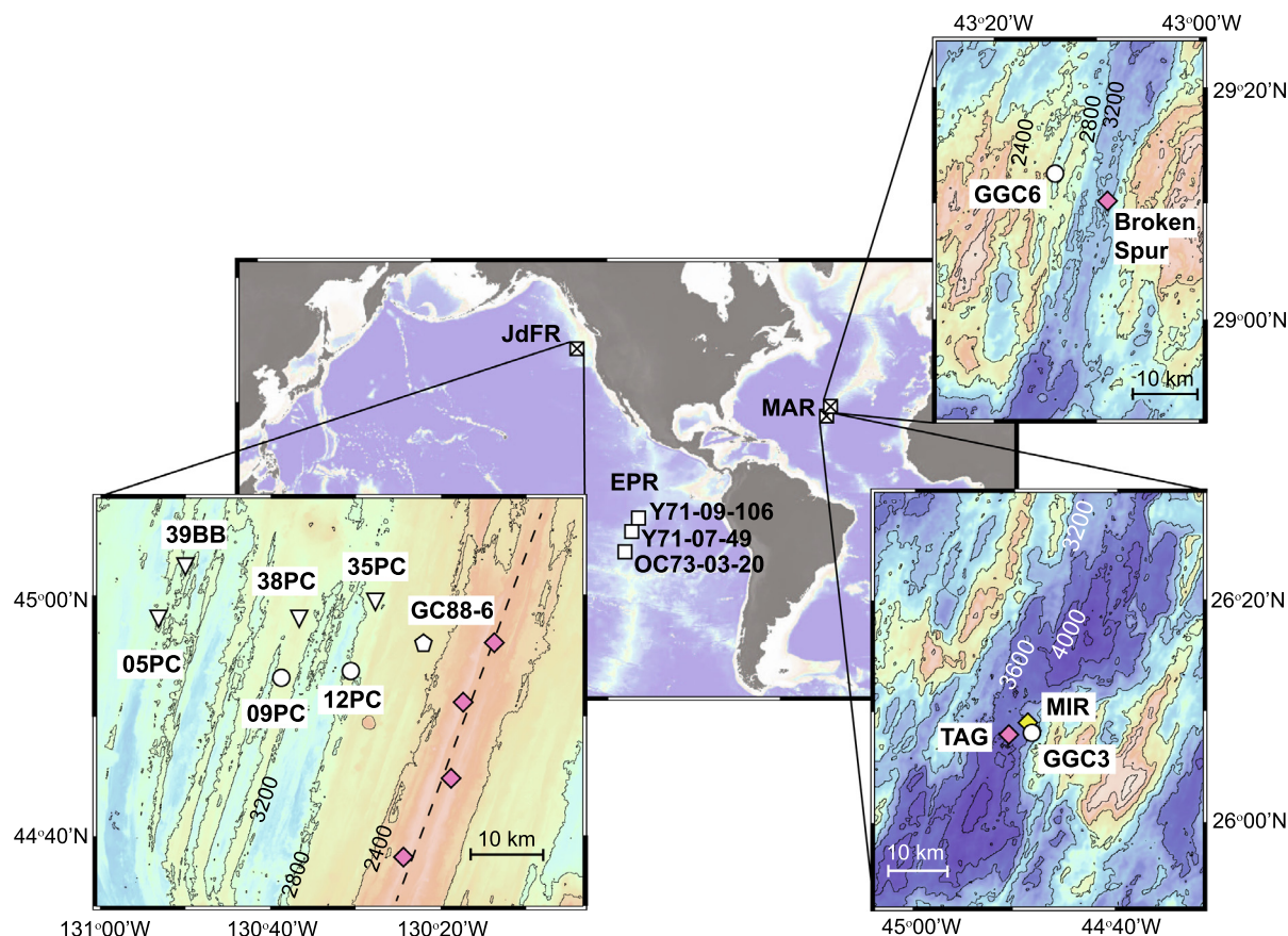
Fig. 1. Locations of sediment cores examined in this work (circles). Study regions on the Mid-Atlantic Ridge (MAR; KN207-2-GGC3 and KN207-2-GGC6) and the Juan de Fuca Ridge (JdFR; AT26-19-09PC and AT26-19-12PC) are highlighted in insets. Diamonds indicate known locations of active (pink) and inactive (yellow) hydrothermal vent fields (Beaulieu et al., 2013). Dashed line depicts position of the Cleft Segment spreading axis. Locations of additional SeaVOICE cores (AT26-19-05PC, -35PC, -38PC, -39BB; triangles; Costa and McManus, 2017) and GC88-6 (pentagon; German et al., 1997) on the Cleft Segment of the Juan de Fuca Ridge, as well as Y71-09-106, Y71-07-49, and OC73-3-20 on the East Pacific Rise (EPR; Lund et al., 2019) are also indicated for reference. Bathymetric contours are spaced at 400 m intervals. Global map and insets generated in GeoMapApp. (For interpretation of the references to colour in this figure legend, the reader is referred to the web version of this article.)
