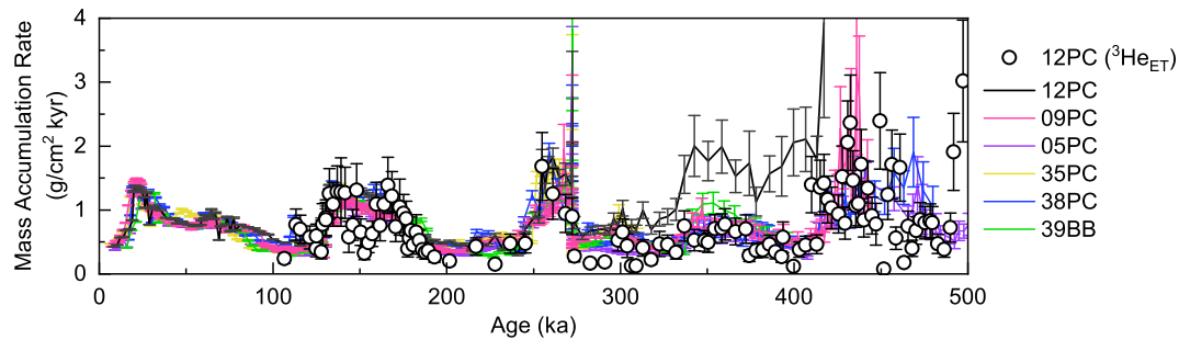
Fig. 9. Comparison of ^3\text{He}_{\text{ET}} -derived (open circles) and ^{230}\text{Th}_{\text{XS}} -derived (black line) mass accumulation rates from 12PC on the Juan de Fuca Ridge with ^{230}\text{Th}_{\text{XS}} -derived mass accumulation rates of neighboring SeaVOICE cores (05PC, 09PC, 35PC, 38PC, 39BB; color lines; Costa and McManus, 2017). In sediments older than 300 ka, ^{230}\text{Th}_{\text{XS}} -derived mass accumulation rates are significantly higher in 12PC than in neighboring cores, but ^3\text{He}_{\text{ET}} -derived values from 12PC are not. SeaVOICE core locations are indicated in Fig. 1. (For interpretation of the references to colour in this figure legend, the reader is referred to the web version of this article.)
